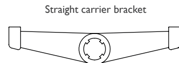
Plan view of LS2-30A bracket
